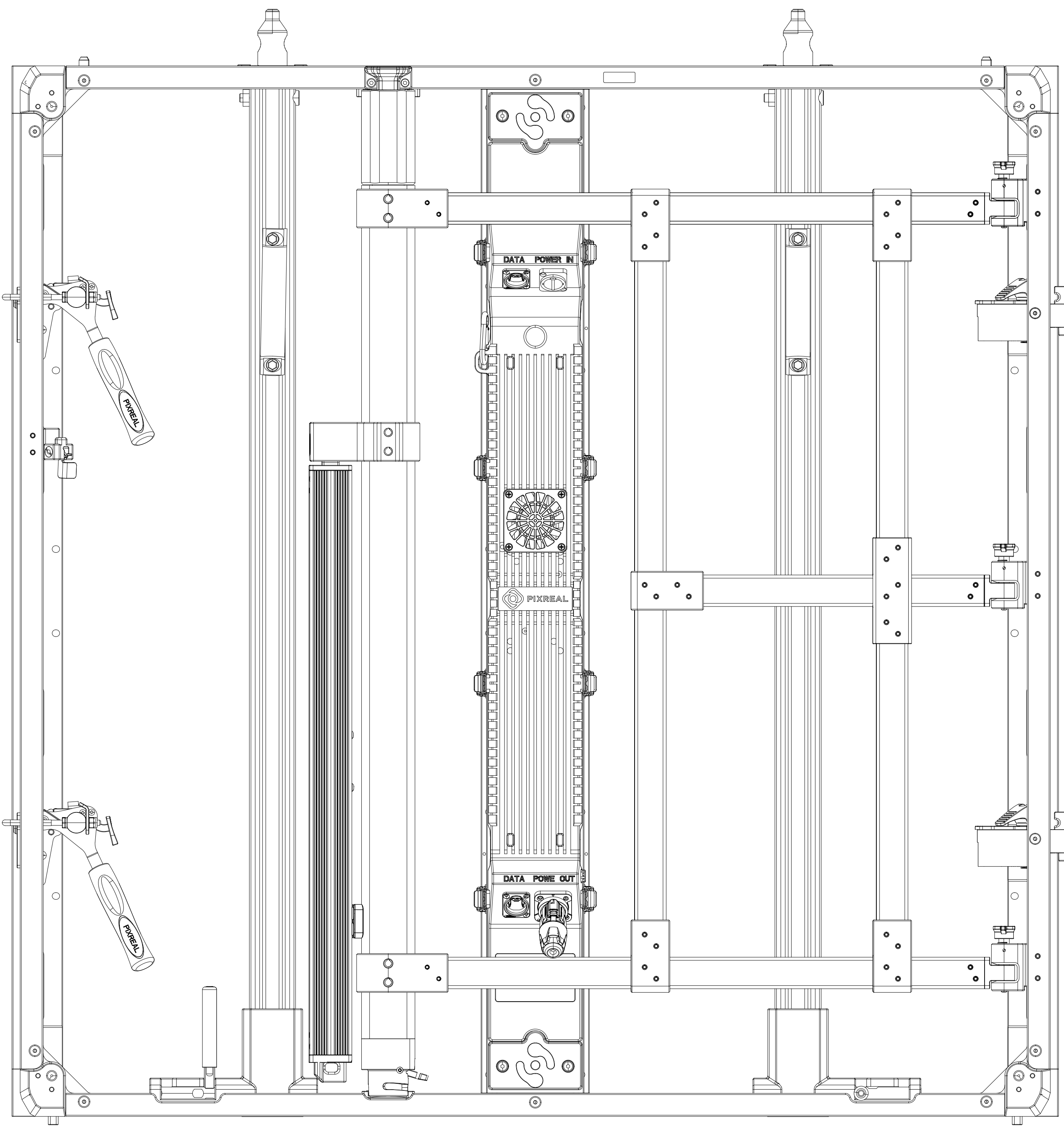
Rear view
