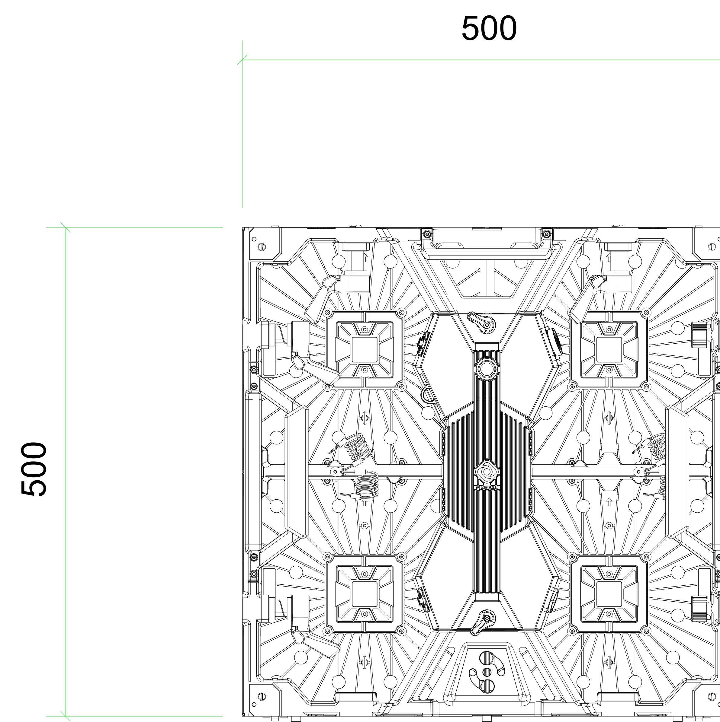
Rear view
